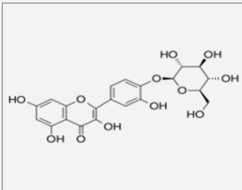
Figure 1: Isoquercetin.
